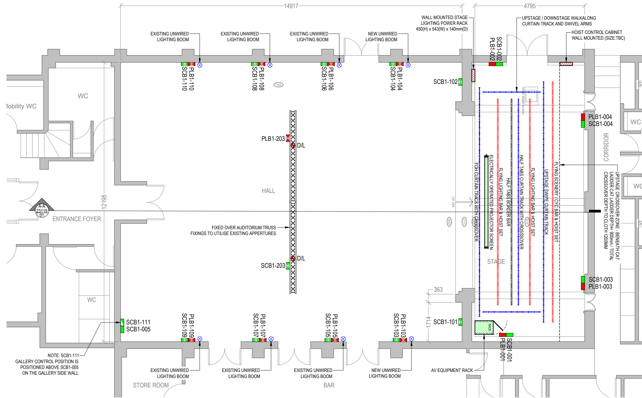
01 HALL & STAGE GROUND FLOOR OVERVIEW PLAN 1:100
