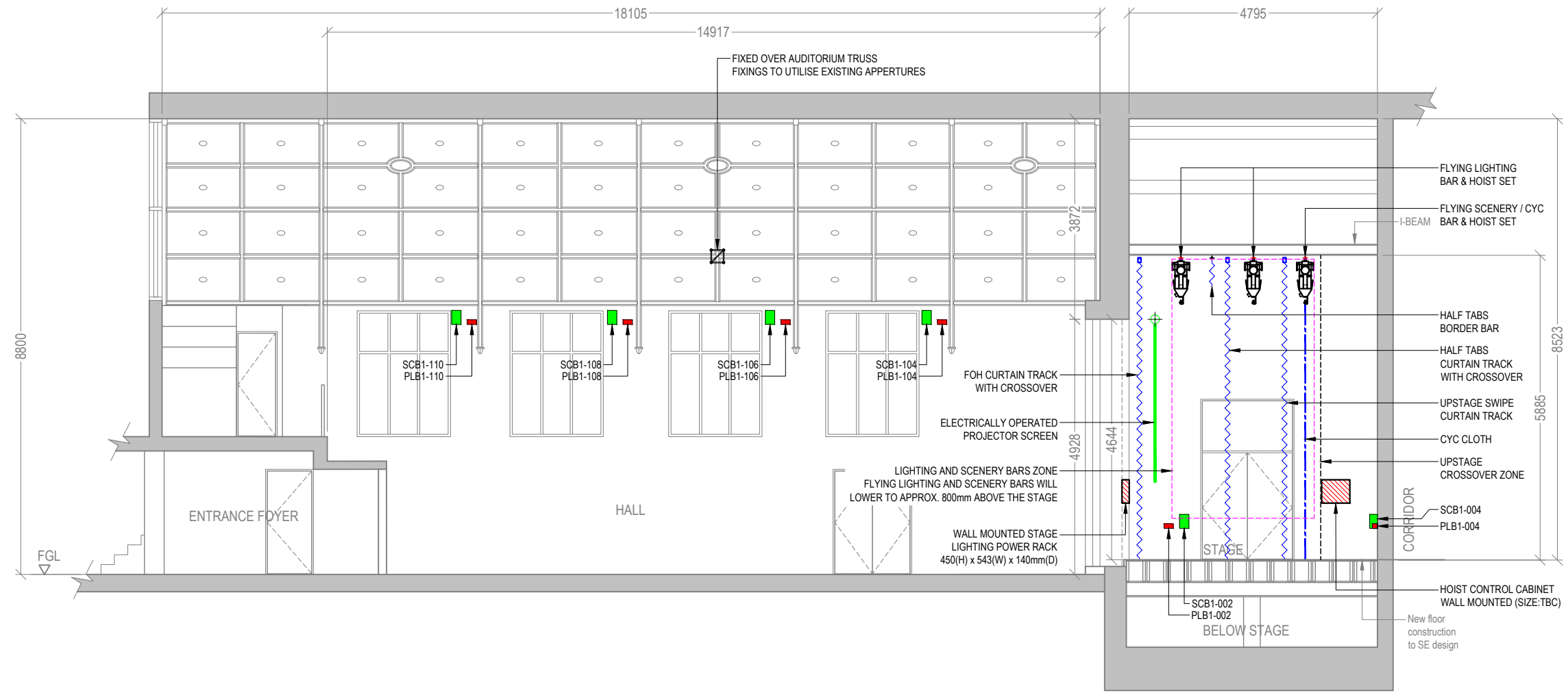
01 HALL & STAGE SECTION A-A 1:100
